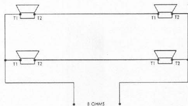
FIGURE 4 — Connection of four 8 ohm speakers in series — parallel
